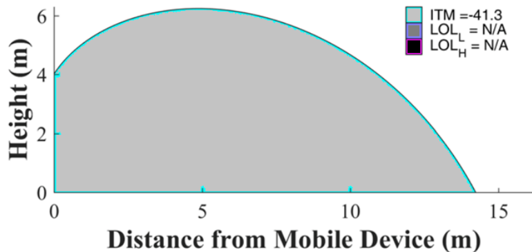
Figure I-140: Handset (EIRP = 23 dBm), Bounding TIM, 1630 MHz
