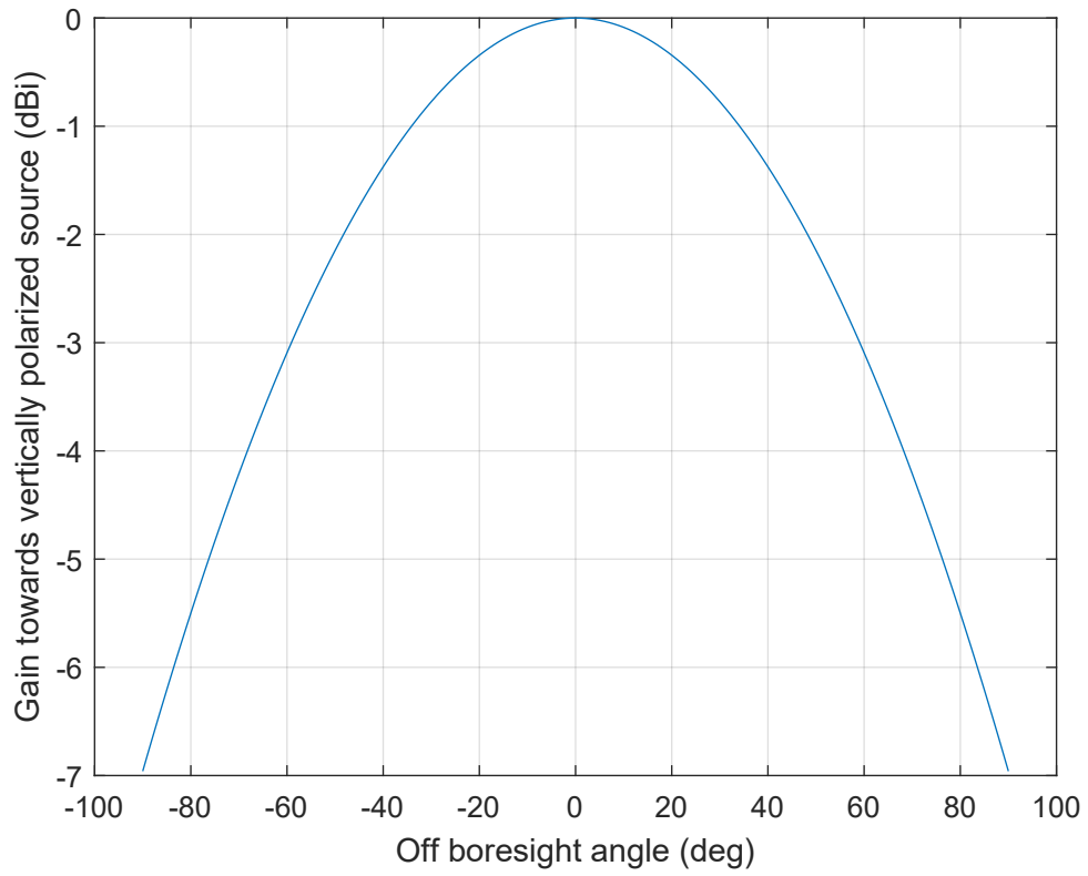
Figure 1. Representative HPR Antenna Gain Pattern towards Vertically Polarized Source [FR Doc. 2024-30760 Filed: 12/26/2024 8:45 am; Publication Date: 12/27/2024]
