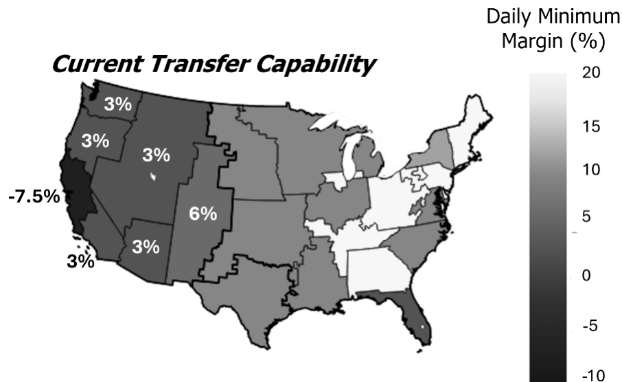
Figure 7.1: Resource Saturation in the Western Interconnection, September 6, WY2022 (2033 Case)
