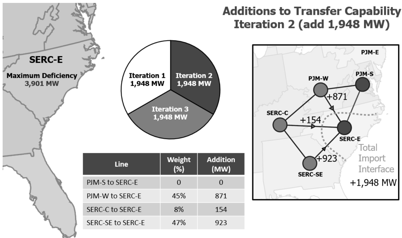
Figure 6.7: SERC-E Iteration 2 Allocation of Additional Transfer Capability (2033 Case)
