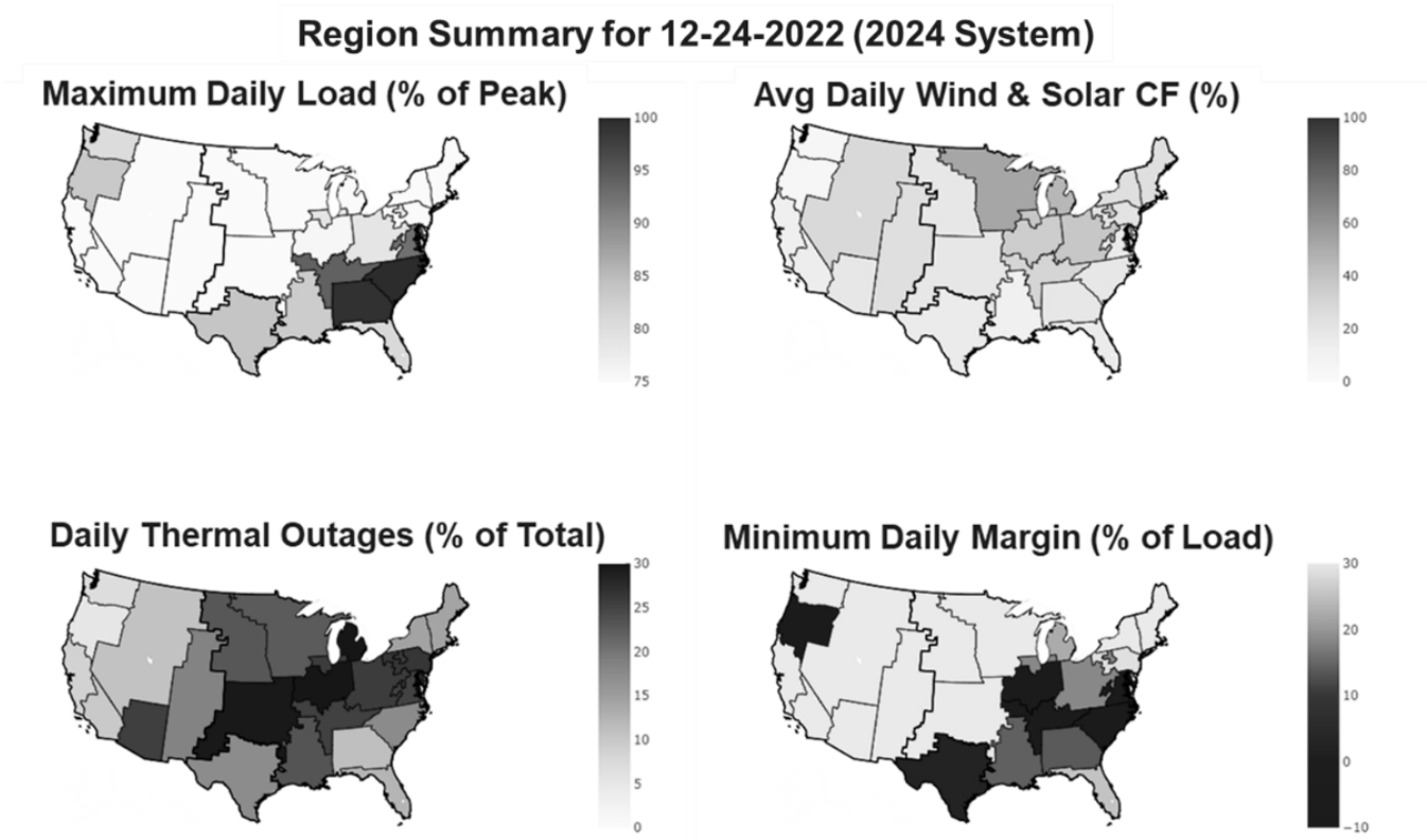
Figure 6.2: Example of Correlated Load, Renewable Output, Weather-Dependent Outages, and Hourly Energy Margin
