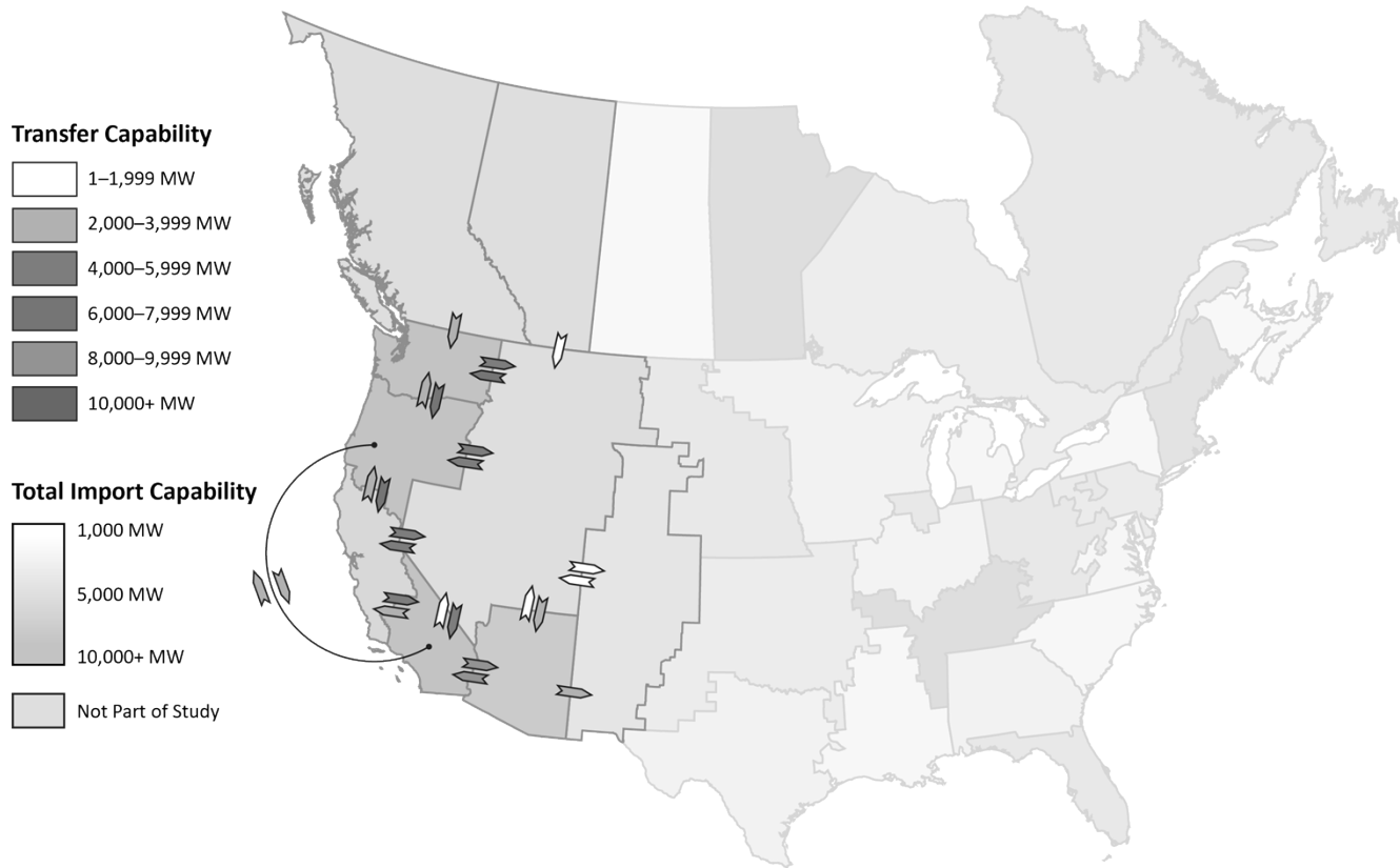
Figure 4.2: Transfer Capabilities for Western Interconnection Interfaces (Winter) Interface W1: British Columbia -> Washington
