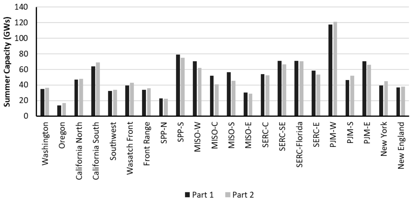
Figure D.3: Comparison of Capacity by TPR, Part 1 vs. Part 2 (2024) 151
