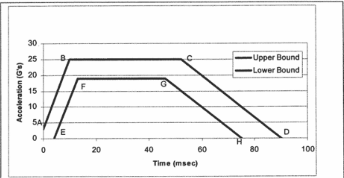
Figure 2 to § 571.213b
