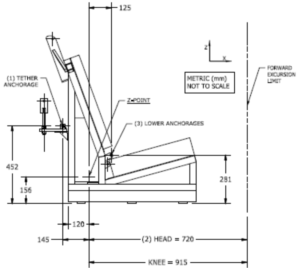
Figure 1B-2 to § 571.213b – Location of the Child Restraint Anchorages and Forward Excursion Limits on the Standard Seat Assembly (See drawing package referenced in this standard for tolerances)
