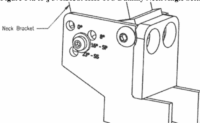
Figure 14a to § 571.213b. HIII-10C Dummy Neck Angle Setting is SP-16 Degrees
