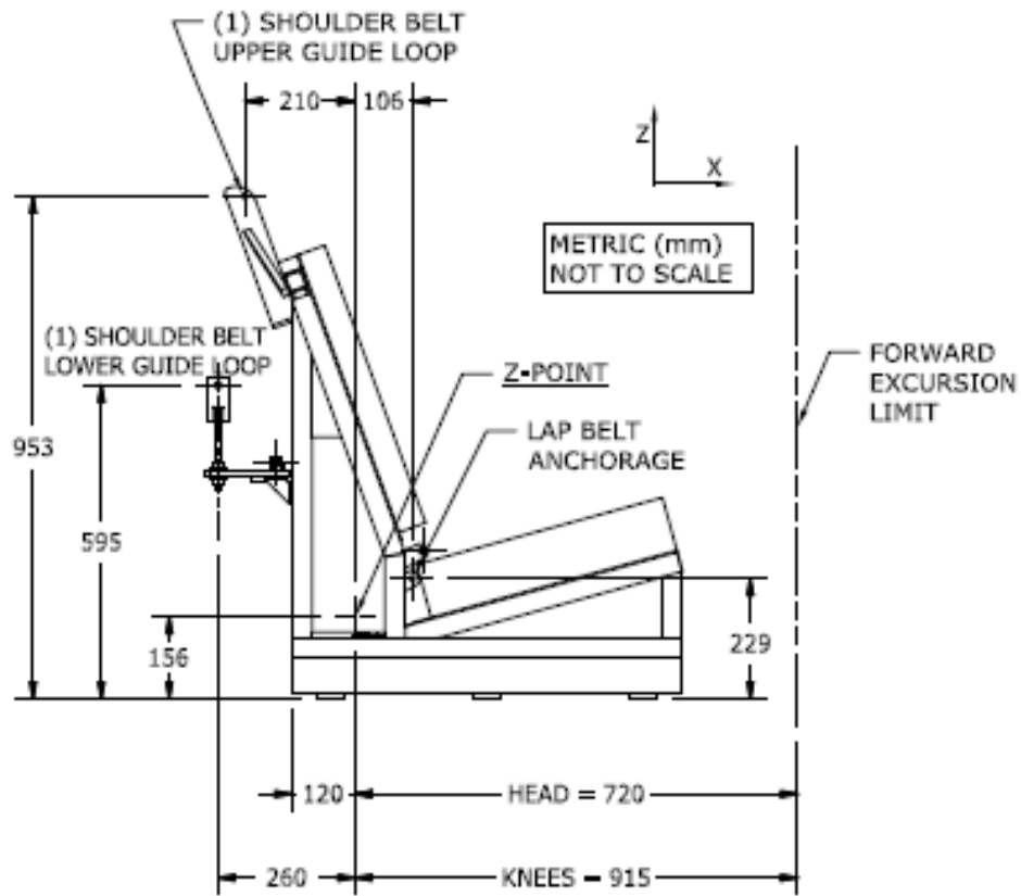
Figure 1B-1 to § 571.213b – Location of Shoulder Belt Upper and Lower Guide Loops and Forward Excursion Limits on the Standard Seat Assembly (See drawing package referenced in this standard for tolerances)
