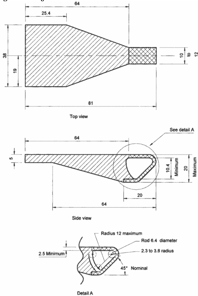
Figure 11 to § 571.213b – Interface Profile of Tether Hook
