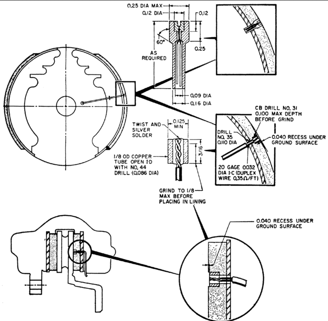
Figure 2. Typical Plug Type Thermocouple Installations
